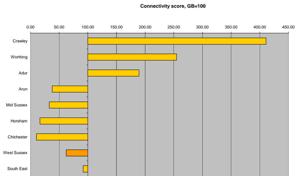
Figure 36: Connectivity Score
